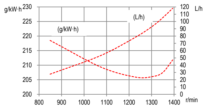
— Full load speed characteristics - - - Propeller characteristics
